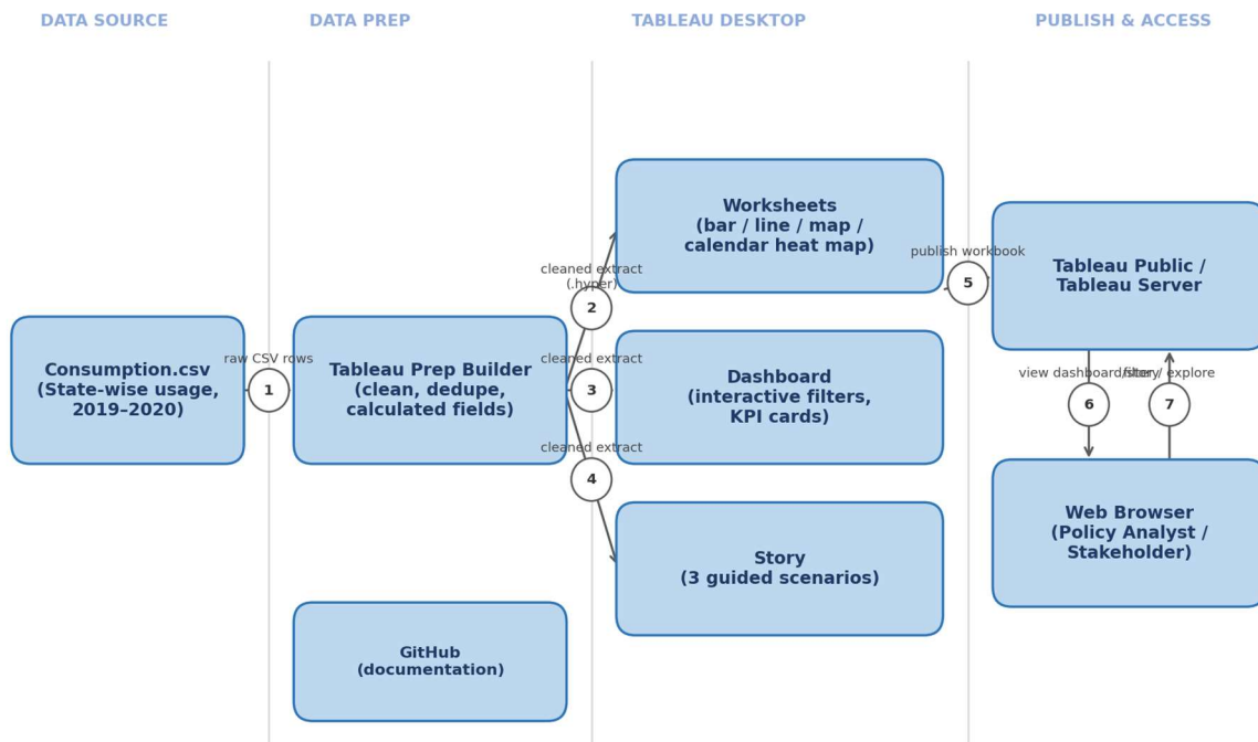
Figure 1: Architecture and data flow of the electricity consumption analytics platform
